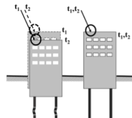
Inter-structural deformation
