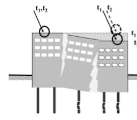
Intra-structural deformation
