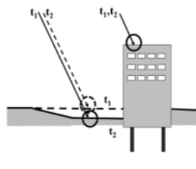
Shallow compaction
